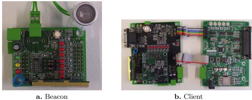
Fig. 3. The components of our location system are equipped with a radio module and an ultrasound transducer
