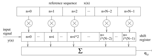
Fig. 6. Correlator
